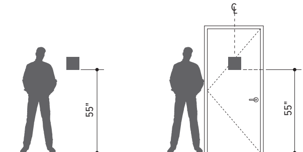
Installation Context - Wall Scale: 3/16" = 1'-0"
